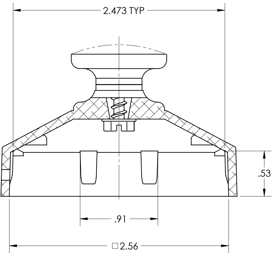
DETAIL K SCALE 3 : 2
